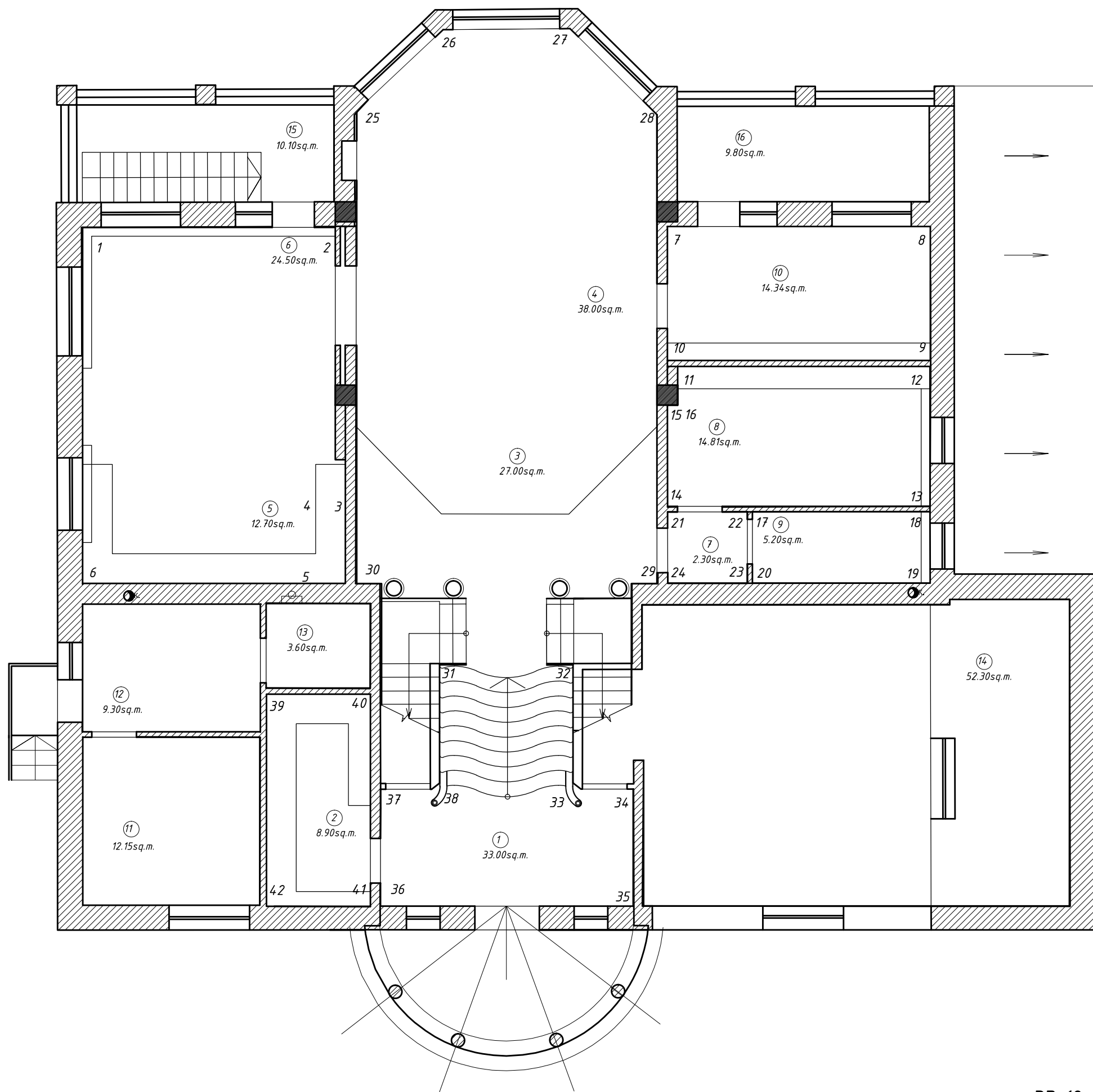
DP -18 Wall denomination scheme 1st floor
