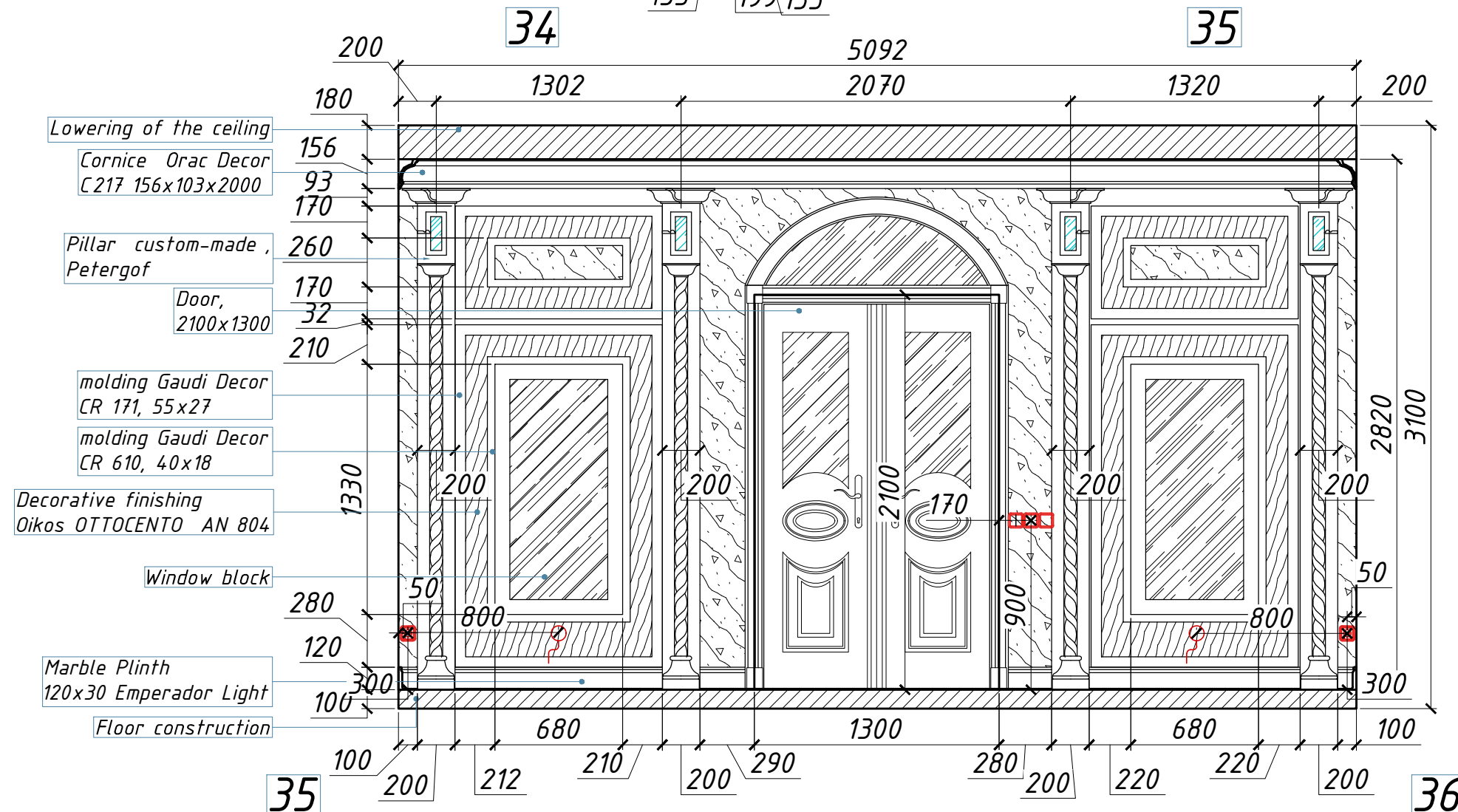
DP -25.1 Wall scheme: Hall, 1st floor (Part 2)
