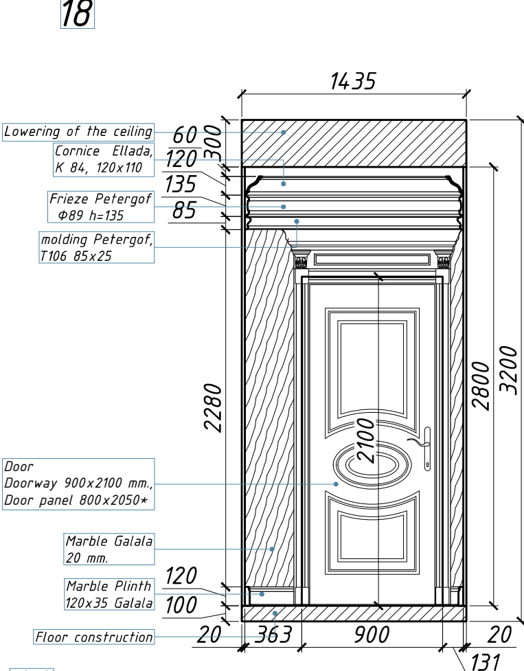
DP -22 Wall scheme: Bathroom, 1st floor (Part 1)
